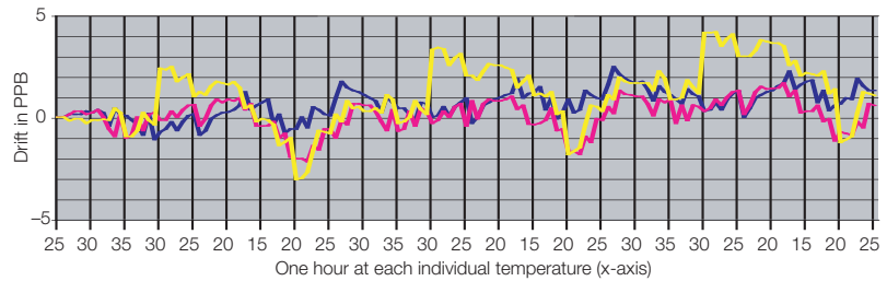
Typical frequency accuracy of the MT8222A for 24 hours following the GPS antenna disconnect over temperature range 15° C to 35° C.
